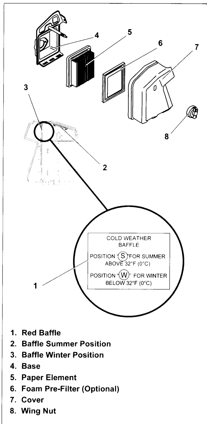
Figure 25. Air Cleaner and Optional Anti-Icing Baffle
