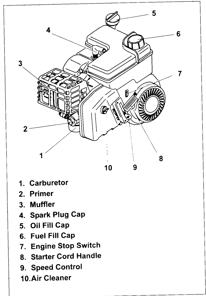
Figure 14. Engine Components
